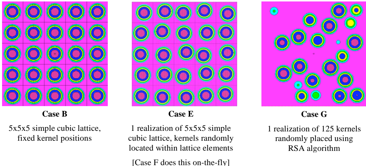
Figure 2. Geometry for MCNP5 calculations of fuel kernels in graphite matrix
