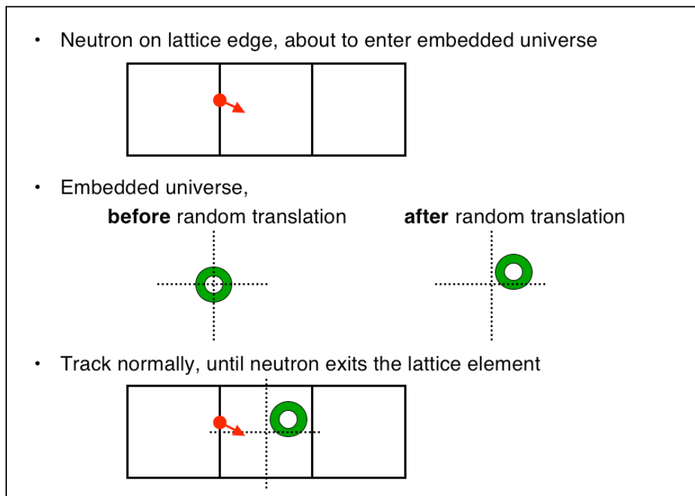
Figure 1. Illustration of MCNP5 Stochastic Geometry Treatment
