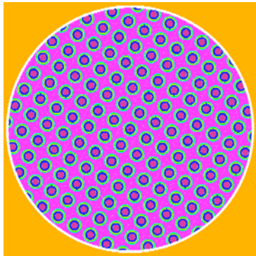
3a. Infinite lattice of fuel kernels, with partial kernels due to clipping by the enclosing cylinder
