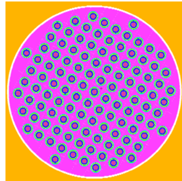
3b. Finite lattice of fuel kernels, with graphite matrix in lattice elements which intersect the enclosing cylinder
