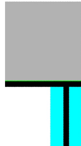
Figure 2. Detail of cross section of wall and ceiling.
